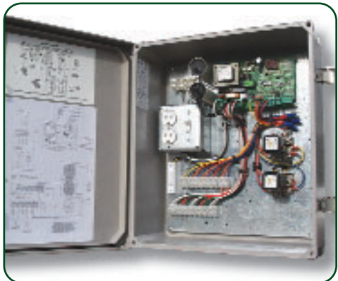
Model 455 D Control Panel shown in pre-wired hinged, lockable enclosure
